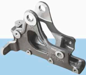
CODE NO. : SHBC 653 PART NAME : PIVOT ARM BRACKET RH (CASTING) VEHICLE : ALL PRIMA TIPPER / TRACTOR MO PART NO. : 2816 8910 3715
