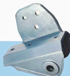
CODE NO. : SHBC 413 PART NAME : FRONT SPRING FRONT BRACKET (LH) (CASTED) VEHICLE : TATA 407 PART NO. : 2651 3210 0123
