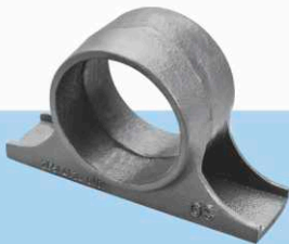
CODE NO. : SHBC 271 PART NAME : CENTRE BEARING BRACKET (CASTED) VEHICLE : TATA 407 PART NO. : 2651 4130 0101
